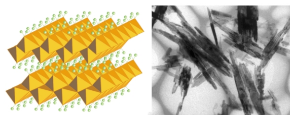
Fig. 5 Crystal structure of lepidocrocite \gamma\text{-FeOOH} and image of particles resulting from oxidation of \text{Fe}(\text{OH})_2 .
