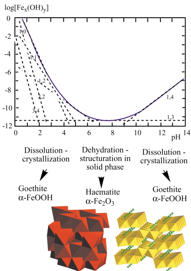
Fig. 6 Influence of pH on the solubility of iron and ferric (hydro)oxide crystal structures.
