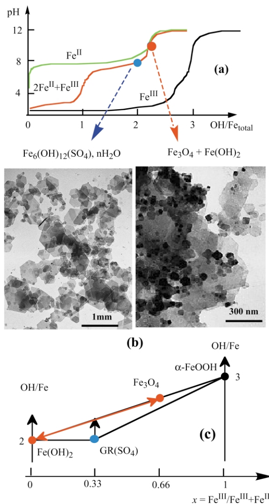
Fig. 10 pH titration curves of Fe(II), Fe(III) and a Fe(II)–Fe(III) mixture ( x = 0.33) (a). Electron micrographs of products formed for OH/Fe total = 2 and at the equivalent point (OH/Fe total = 2.34) (b). Phase diagram showing the relation between GR, ferrous hydroxide and magnetite during alkalization. Adapted from (23).
